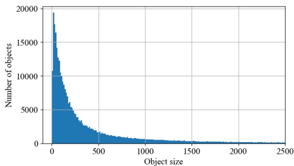
Fig. 3. Distribution of object sizes in training dataset
